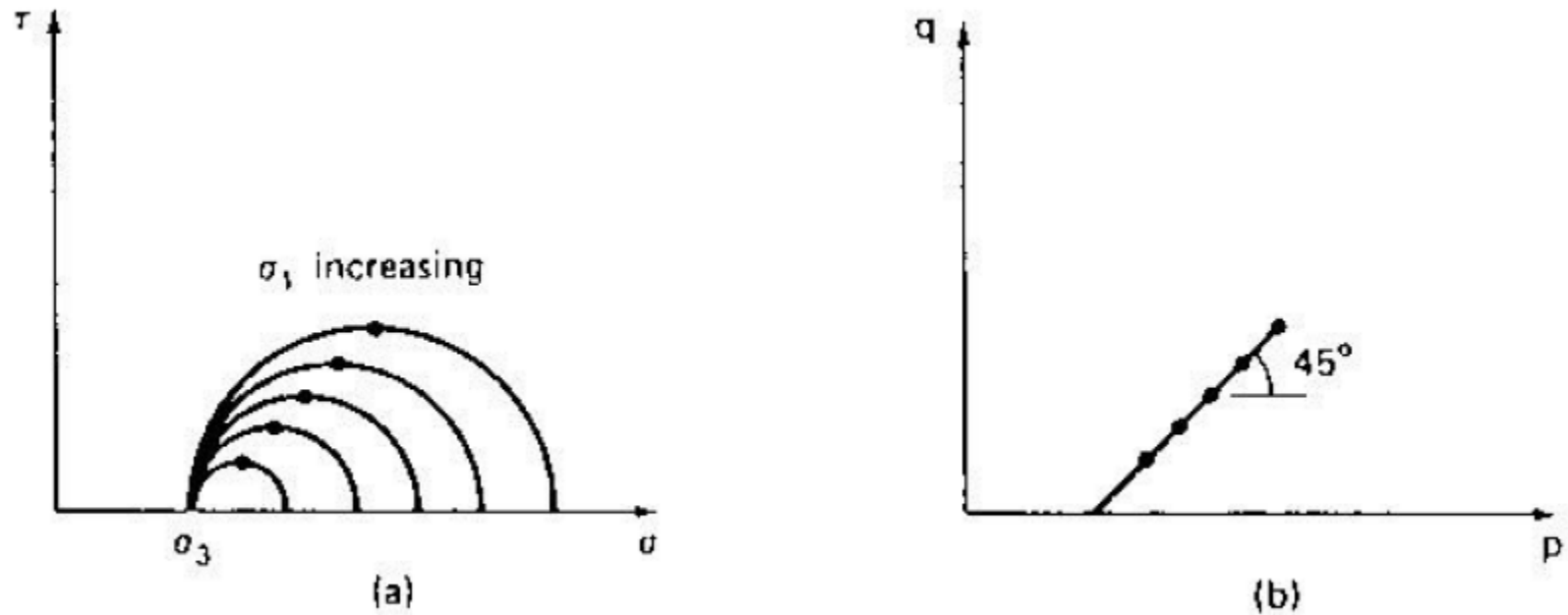
(a) Successive Mohr circles; (b) stress path for constant \sigma
