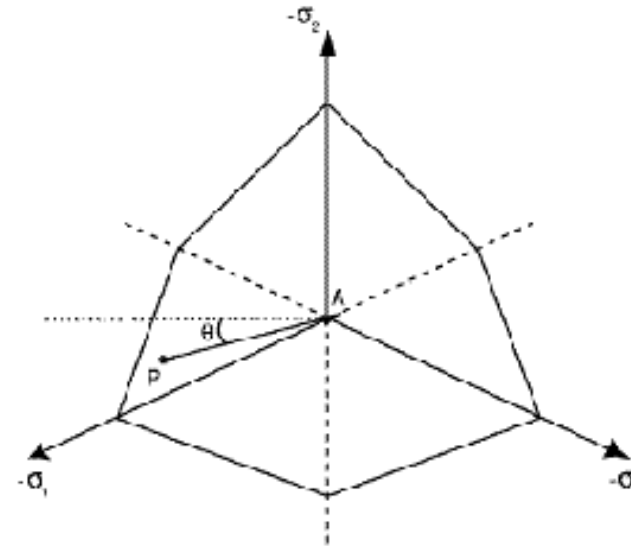
\Pi plane
